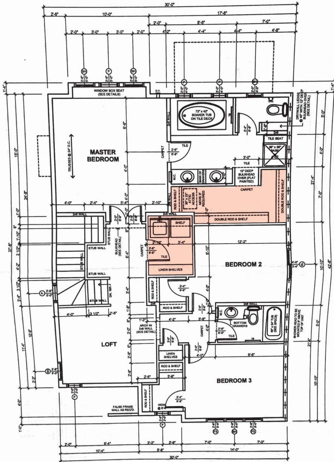
SECOND FLOOR 1236 Sq. Ft.
